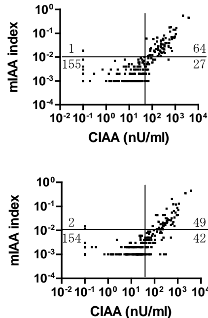
図1 New RIA assay (上図) and previous RIA assay (下図) (Babaya N, et al., Diabetes Metab Res Rev 25, 665-670, 2009より引用)
