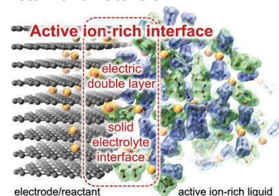
Figure 3. Active ion-rich interface (reaction field).
