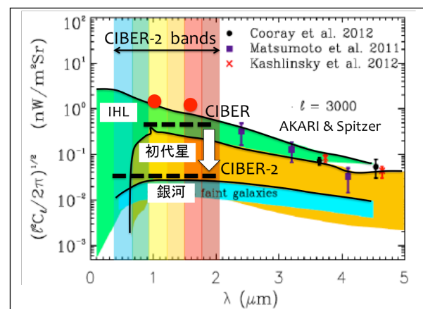
Figure 1 spectrum
