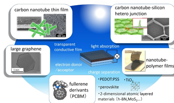
Fig. 2 Nano-carbon energy devices.
