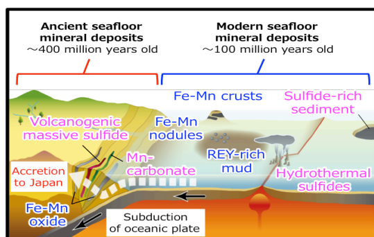
Fig. 1 Modern and ancient seafloor mineral deposits
