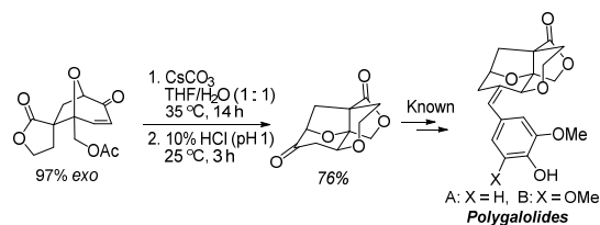
Scheme 8. Conversion to polygalolide intermediate
