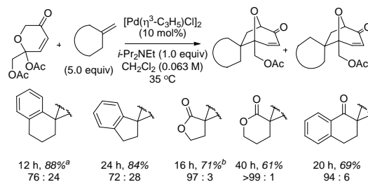
Scheme 7. Scope of Pd-catalyzed [5+2] cycloadditions with exocyclic methylenes
