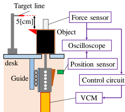
(b) Configuration of the system
