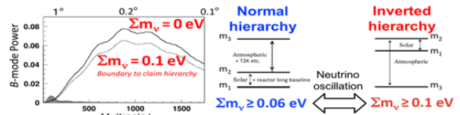
Figure 2 Measurements of \Sigma m_\nu , potentially determine mass hierarchy of neutrino.
