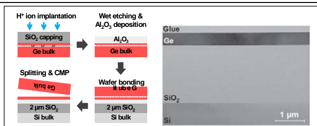
Fig. 2 GOI formation method by smart cut and example of fabricated GOI structure
