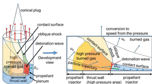
Figure 1 Detonation Engine
