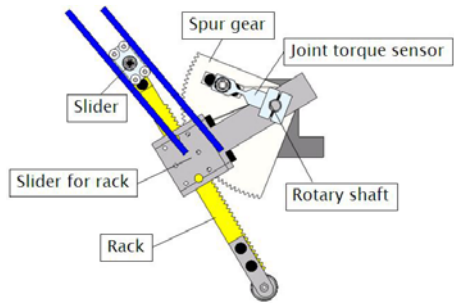
Fig.4 Operation mechanism for fingertip
