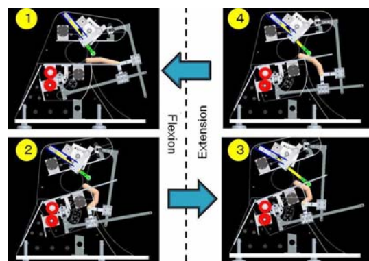
Fig.3 Finger rehabilitating with the proposed device
