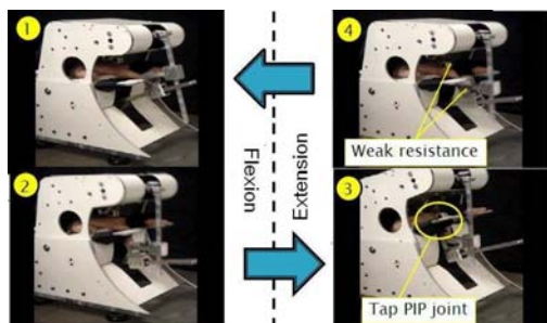
Fig.8 Experiment view
