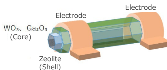
Figure 1 Core-Shell structured gas sensor
