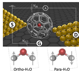
Fig. 1 Schematic illustration of a single molecule transistor structure with a \text{H}_2\text{O}@C_{60} molecule as a quantum dot.
