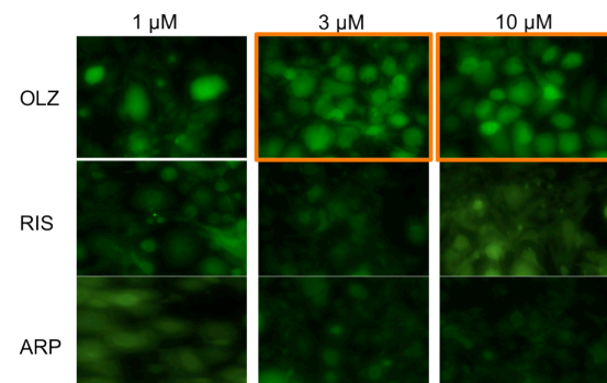
Fig. 2. PPAR \gamma expression in differentiating 3T3L1 cells treated with SGAs for 24 hr. Cells were differentiated with olanzapine (OLZ), risperidone (RIS) and aripiprazole (ARP) for 24 hr and then their PPAR \gamma expression was observed using immunofluorescence technique.
