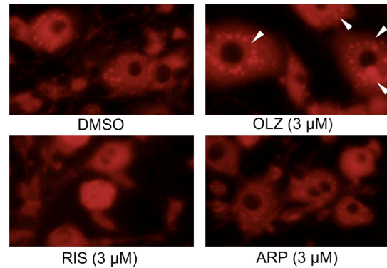
Fig. 1. Nile red staining of differentiated adipocytes. Cells were differentiated for 48 hr and consequently, medium was changed to sustained medium and treated with 3 μM of SGAs for 7 days and then stained with Nile Red (5 μg/mL).
