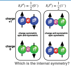
Figure 2. Two possible internal structures of the simplest kaonic nucleus " K^-pp ", which must be examined experimentally.
