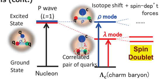
Figure 2. When a quark ( q ) in an ordinary baryon (nucleon) is replaced with a heavy charm quark ( c ), the motions of quarks inside a baryon are separated (isotope shift). The length of the arrow represents the mass difference between the states (excitation energy).
