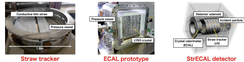
Figure 4. High-sensitive StrECAL detector
