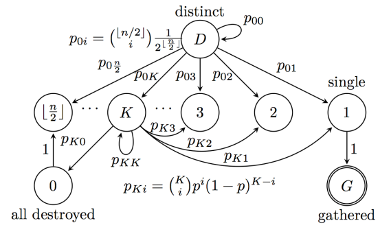
Fig. 2 State transitions of probabilistic gathering with crash faults.
