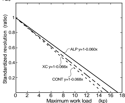
Figure 2. The relationship between standardized revolution ratio and maximum work load at each groups. Standardized revolving scaled was to one maximum speed.
