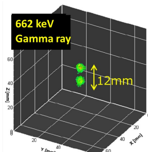
Fig.1: (left) Tri-color image using diced scintillator array (right) 3D gamma-ray image using Compton camera.
