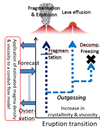
Figure 2 Improvement of eruption models through the observation-forecast-variation cycle
