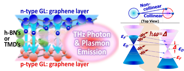
Fig. 2 Photon- and plasmon-assisted resonant tunneling in the G-DGLs for THz emitters.
