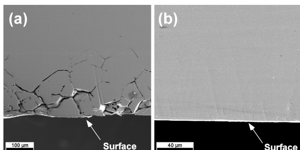
Fig.1 Effect of grain boundary control on corrosion in austenitic stainless steel (SUS304): (a) Conventionally processed, (b) grain boundary engineered. (S.Tsurekawa et al. , Acta Mater. , 54,3617, (2006).)
