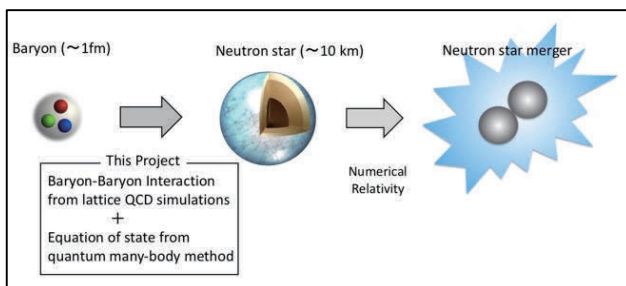
Figure 1 From quarks to neutron star mergers
