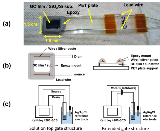
Figure 1. Schematic configuration of the sensing performance measurement system of solution gated CG FET and extended gate FET pH sensors. (a) The photograph of the sensor chip, (b) Schematic illustrations of the structure of the sensor chip for the top view and the cross-sectional view, (c) the measurement system for the solution top gate structure and the extended gate structure.
