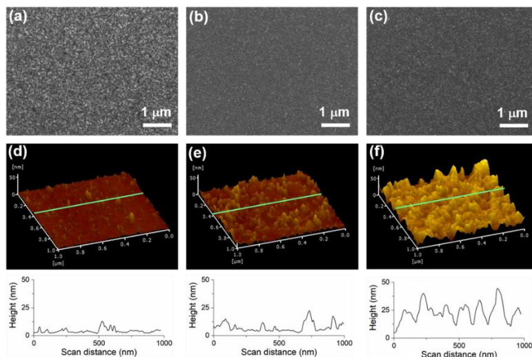
Figure 2. FE-SEM images of glassy carbon films directly grown on \text{SiO}_2/\text{Si} substrate with different growth time; (a) for 10min, (b) for 30min, and (c) for 60min, respectively. AFM images of the samples; (d) for 10min of sample (a), (e) for 30min of sample (b), and (f) for 60min of sample (c), respectively. The bottom insets show scan profiles indicated in the AFM images respectively.
