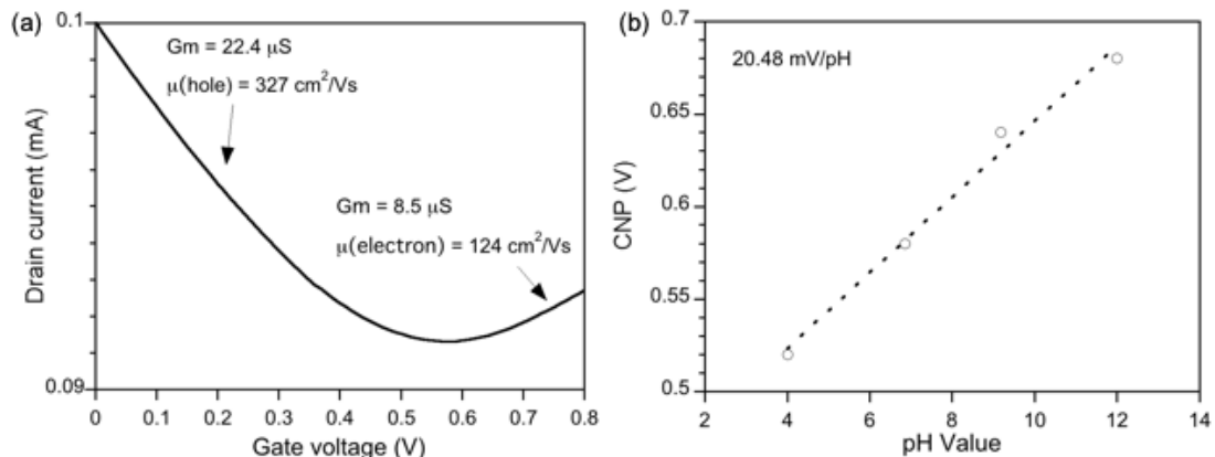
Fig.6 (a) I DS -V G characteristics, (b) CNP shifts in different buffer solution with pH values where a sensitivity of 20.48 mV/pH was obtained.
