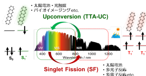
図1 Photon upconversion と Singlet fission
