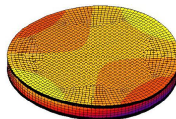
Fig. 9 Out-of-plane deformation of CFRP sandwich structure
