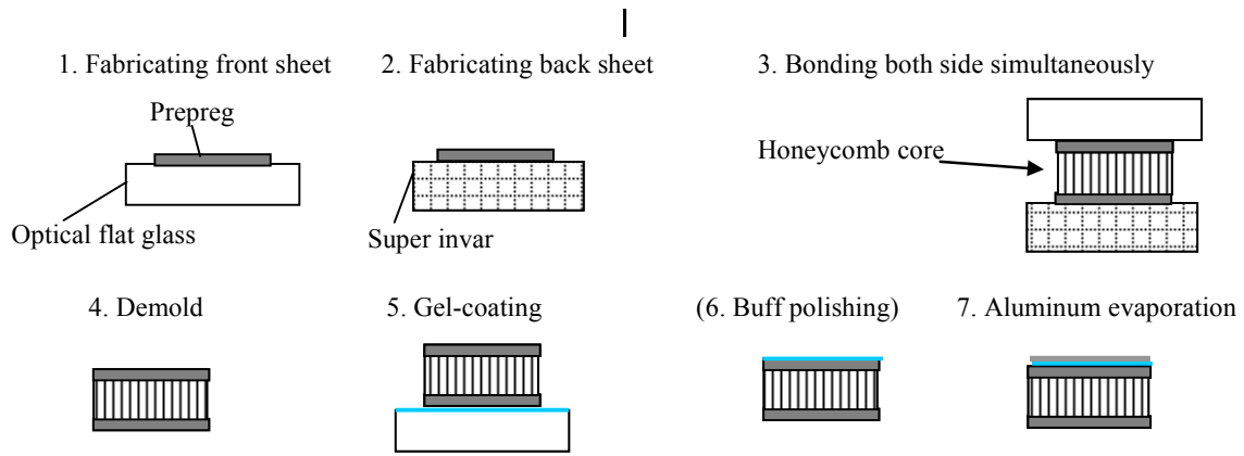
Fig. 3 Fabrication flowchart for CFRP sandwich mirror
