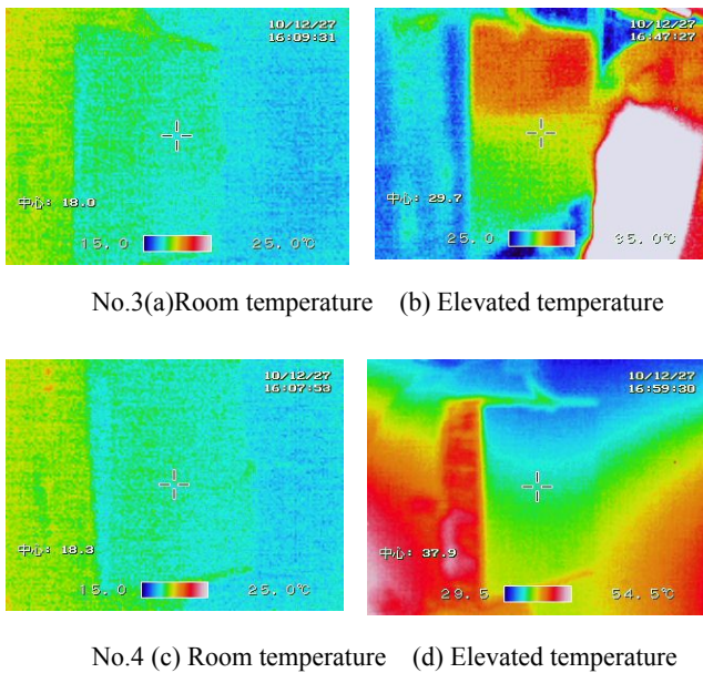
Fig. 7 Temperature distributions at measurements
