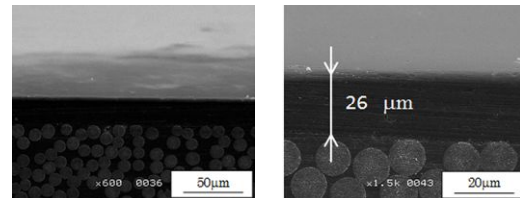
Fig. 2 Gel-coated CFRP plate surface
