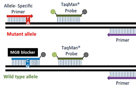
図1 castPCR
